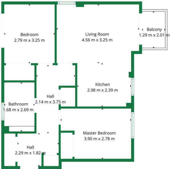
TOTAL: 62 m 2 Ground floor: 62 m 2 EXCLUDED AREAS: BALCONY: 3 m 2 , WALLS: 5 m 2
